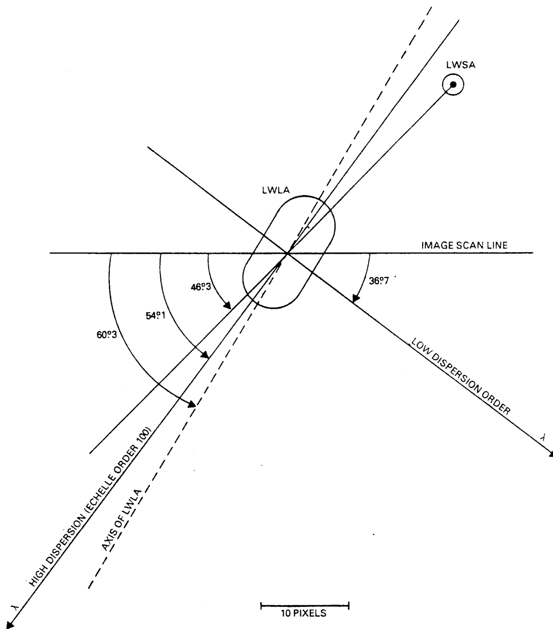
Figure 2.17: LWR Geometry
